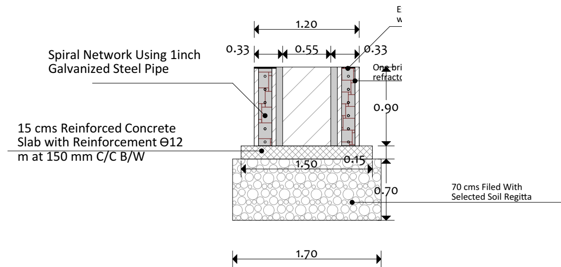
Section B-B
