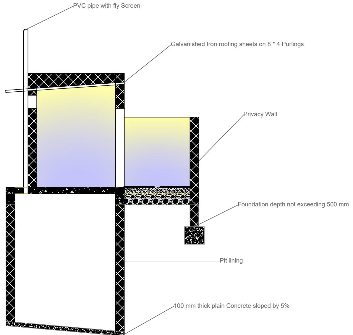
Section Y-Y Detailed
